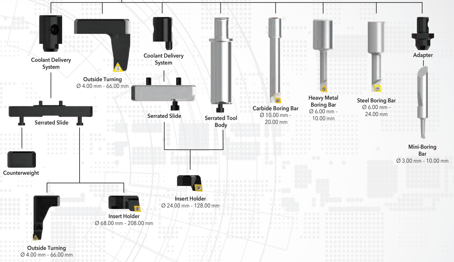
PrimeBore Head
